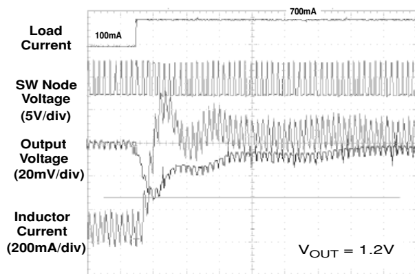
Transient Response
