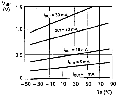
7.3 S-81220SG series
