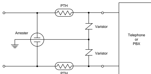
(5) Telecommunication Circuit
