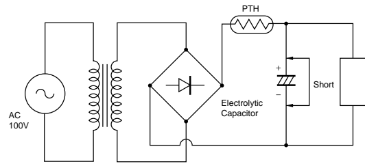
(4) Short - Circuit Test of Electrolytic Capacitor
