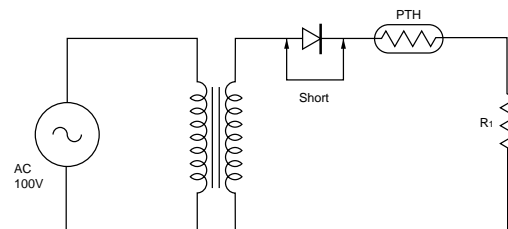
(2) Short - Circuit Test of Diode
