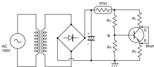
(1) Short - Circuit Test of Transistor
