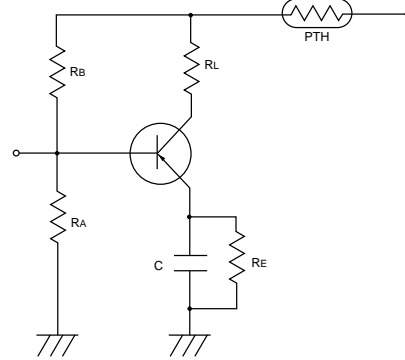
(2) Transistor Protection Circuit
