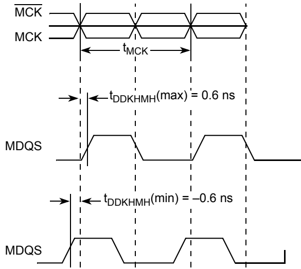
Figure 5. Timing Diagram for t_{\text{DDKMH}}
