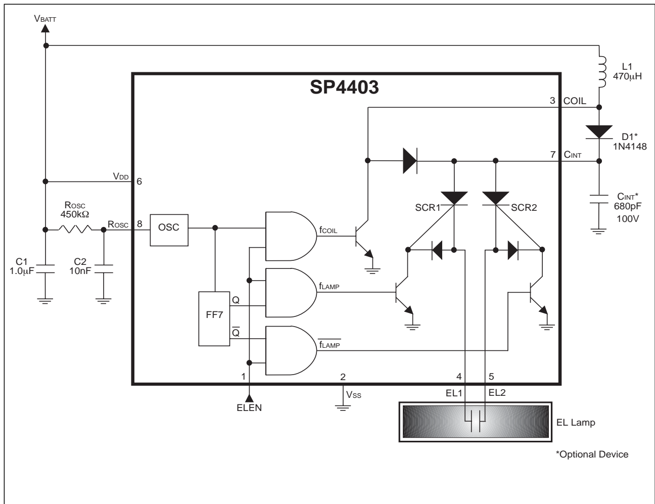
Figure 1: Internal Diagram of the SP4403
