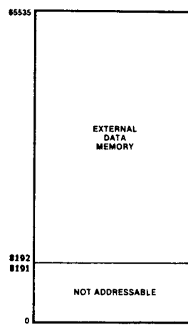
Figure 5. Data Memory Map
