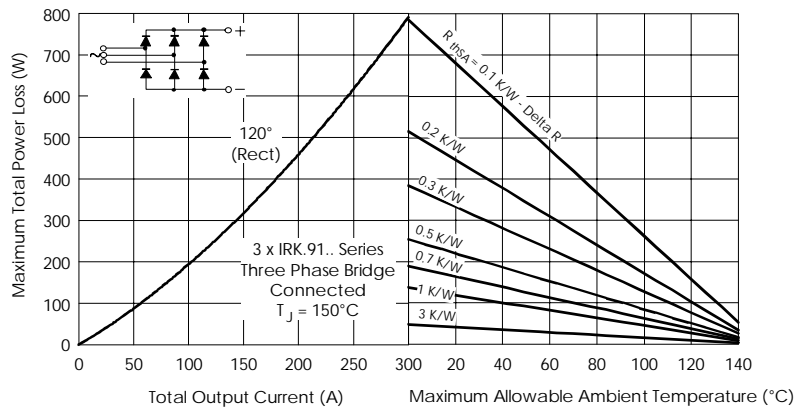
Fig. 9 - Forward Power Loss Characteristics
