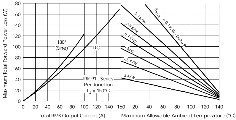
Fig. 7 - Forward Power Loss Characteristics
