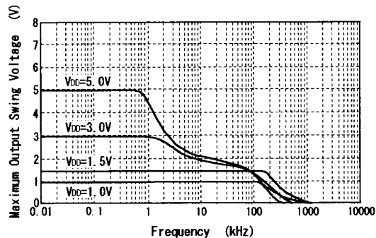
Maximum Output Swing Voltage vs. Frequency
