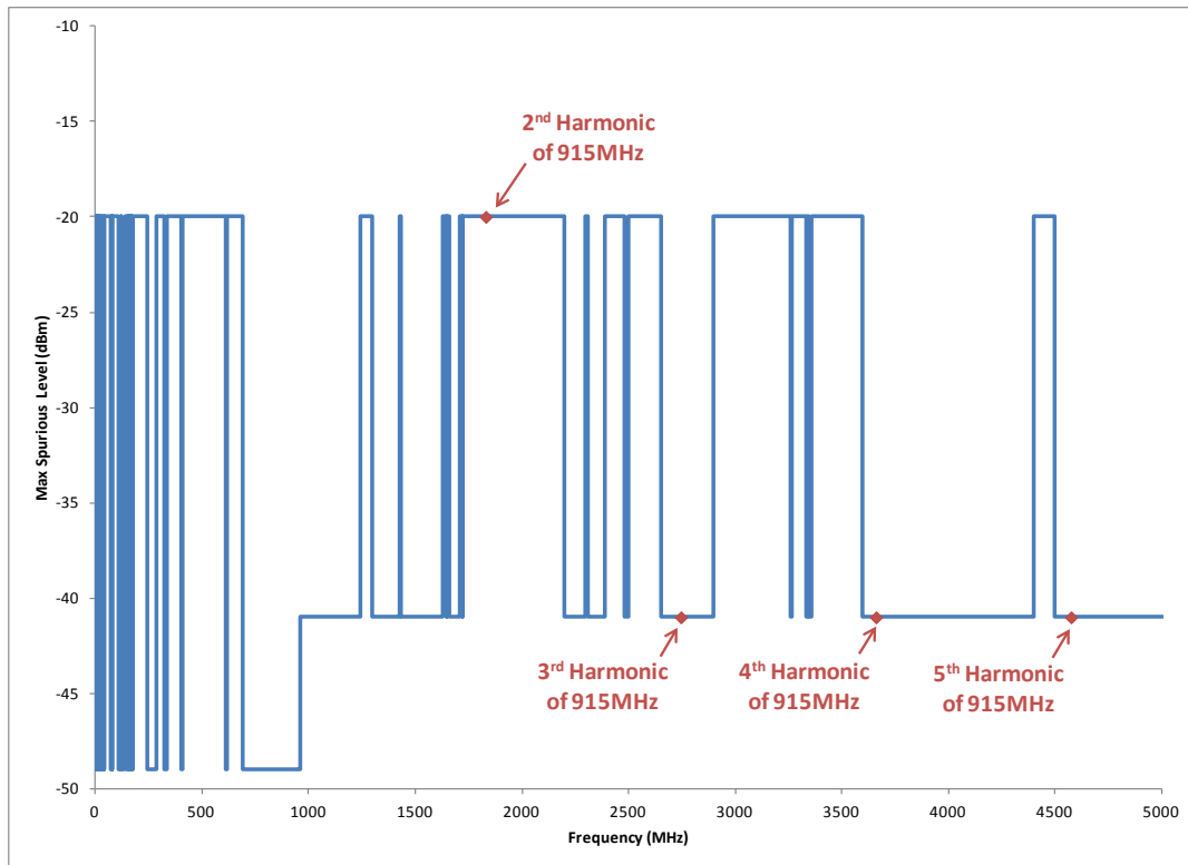
Figure 2. FCC Spurious Level Restrictions by Frequency
