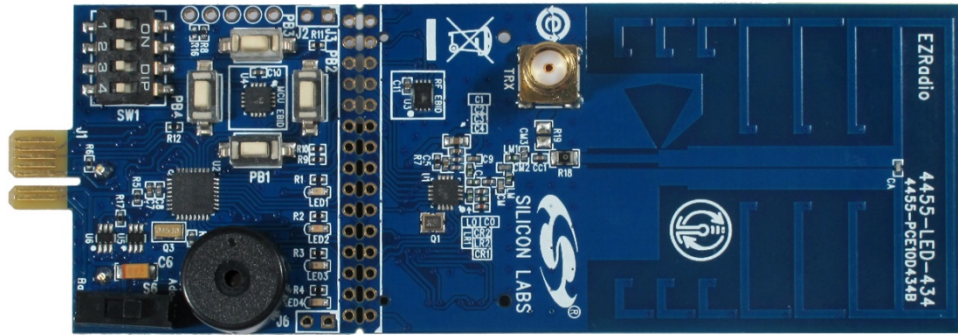
Figure 5. Si4455 EZRadio Demo Board
