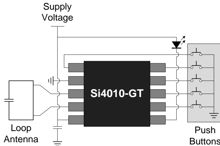
Figure 4. Fully Integrated Transmit Solution (Silicon Labs Si4010 Transmitter)
