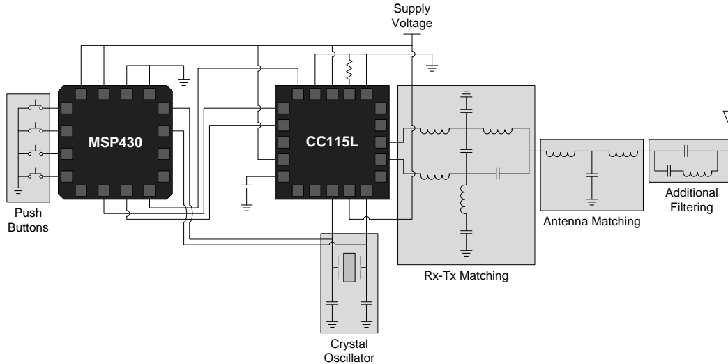
Figure 3. Partial Discrete Transmit Solution (TI CC115L + MSP430)
