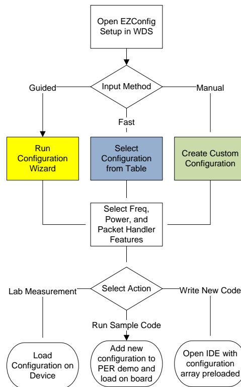
Figure 6. EZConfig Device Configuration Steps
