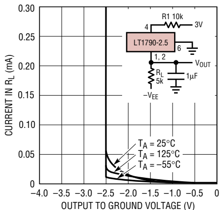
-2.5V Characteristics
