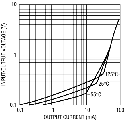
2.5V Minimum Input/Output Voltage Differential vs Load Current
