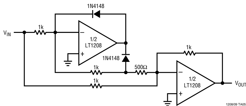
Full-Wave Rectifier
