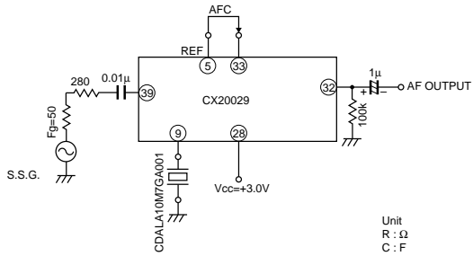
Test Circuit
