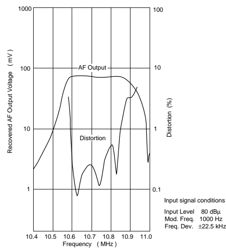
Frequency Characteristics
