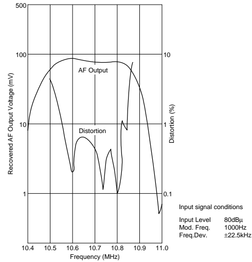
Frequency Characteristics
