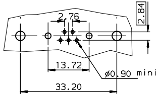
LAYOUT DIMENSIONS (after plating) CONNECTOR SIDE VIEW
