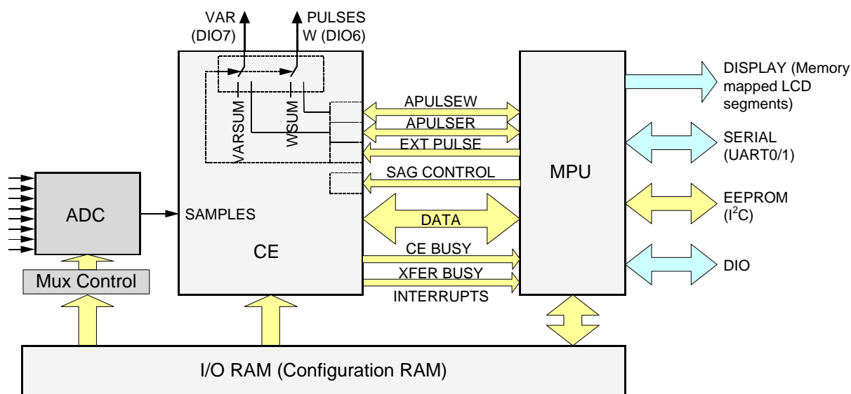
Figure 27: MPU/CE Communication
