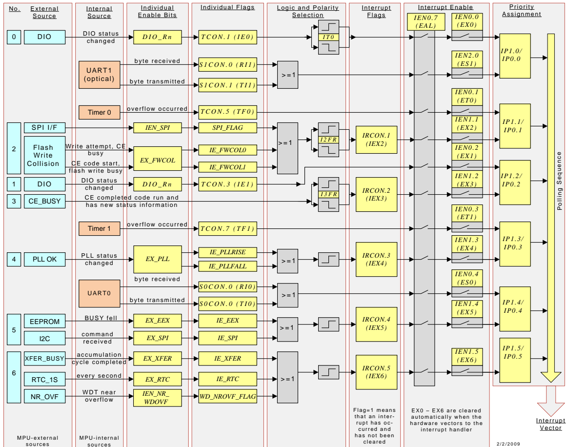
Figure 8: Interrupt Structure
