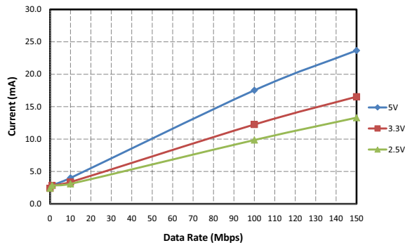
Figure 12. Si8640/45 Typical V_{DD2} Supply Current vs. Data Rate 5, 3.3, and 2.5 V Operation
