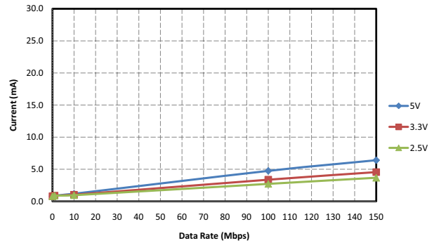
Figure 11. Si8610 Typical V DD2 Supply Current vs. Data Rate 5, 3.3, and 2.70 V Operation (15 pF Load)
