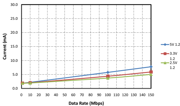
Figure 10. Si8621 Typical V DD1 or V DD2 Supply Current vs. Data Rate 5, 3.3, and 2.70 V Operation (15 pF Load)
