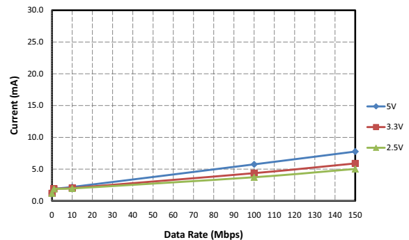
Figure 13. Si8622 Typical V DD1 or V DD2 Supply Current vs. Data Rate 5, 3.3, and 2.70 V Operation (15 pF Load)
