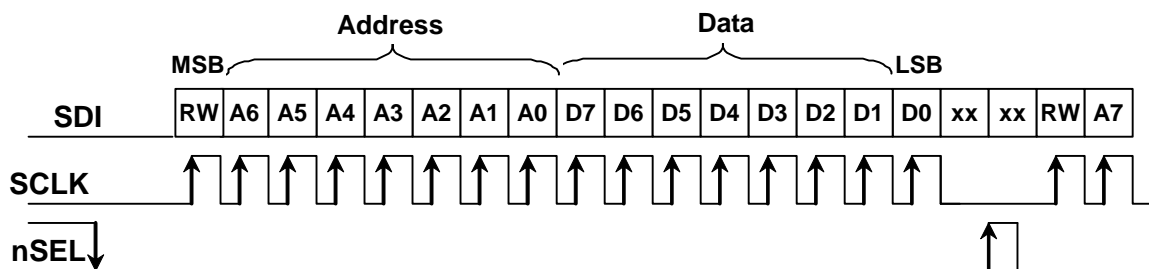
Figure 3. SPI Timing
