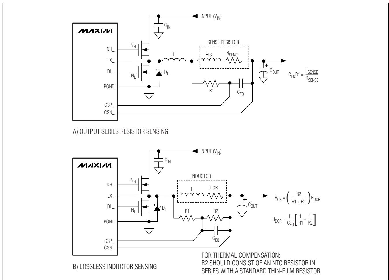
Figure 3. Current-Sense Methods
