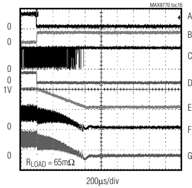
SHUTDOWN WAVEFORMS
