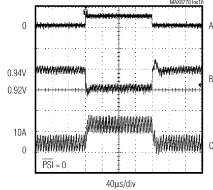
LFM LOAD TRANSIENT ( V_{OUT(LFM)} = 0.9500V )
