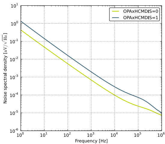
Figure 3.23. OPAMP Voltage Noise Spectral Density (Non-Unity Gain)
