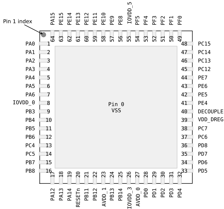
Figure 4.1. EFM32TG840 Pinout (top view, not to scale)
