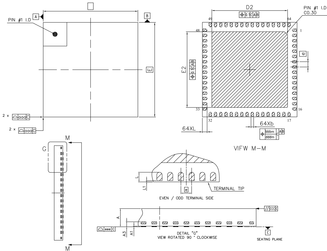
Figure 4.3. QFN64
