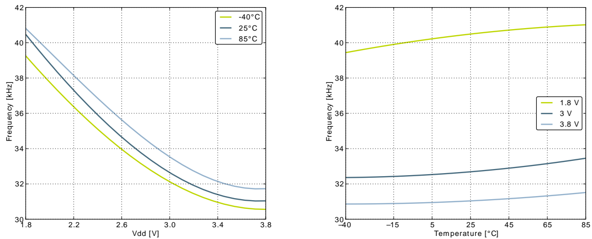
Figure 3.11. Calibrated LFRCO Frequency vs Temperature and Supply Voltage
