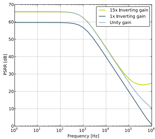
Figure 3.21. OPAMP Negative Power Supply Rejection Ratio
