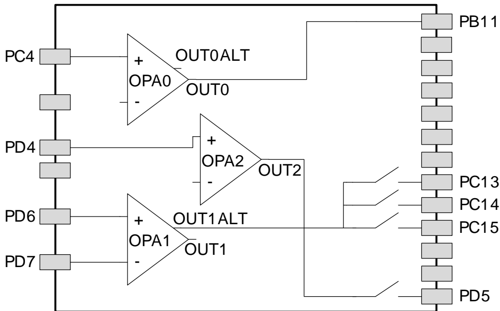
Figure 4.2. Opamp Pinout
