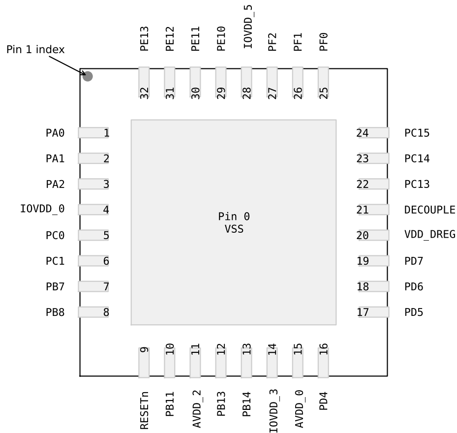
Figure 4.1. EFM32TG210 Pinout (top view, not to scale)
