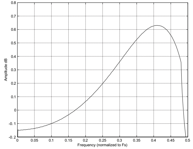
Figure 25. DAC Double-Speed Passband Ripple
