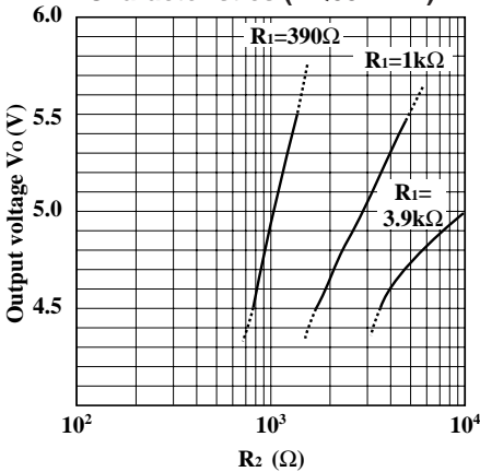
Fig.5 Output Voltage Minute Adjustment Characteristics (PQ05RF2V)
