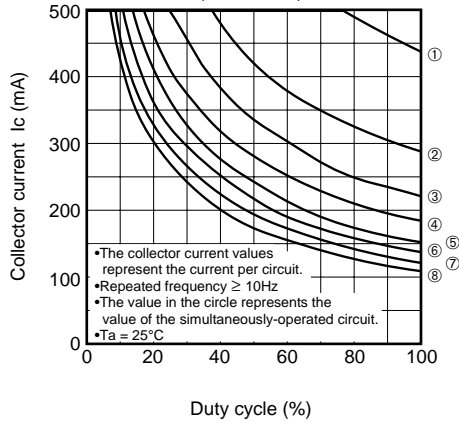
Duty-Cycle-Collector Characteristics (M54585FP)
