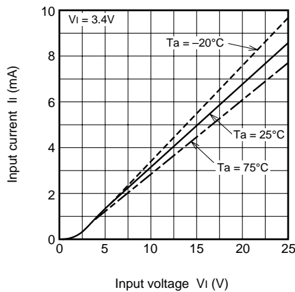
Input Characteristics
