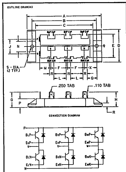
KE721203 Six-Darlington Transistor Module 30 Amperes/1200 Volts
