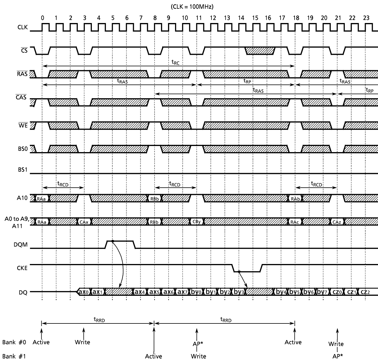
Figure 6. Interleaved Bank Write (Burst Length=8, Auto Precharge)
