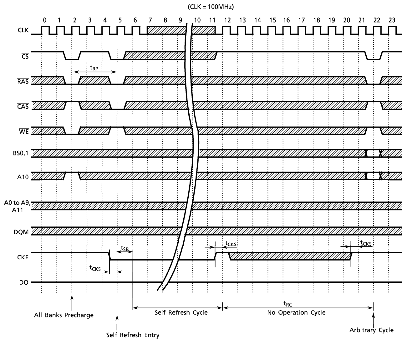
Figure 12. Self Refresh Cycle
