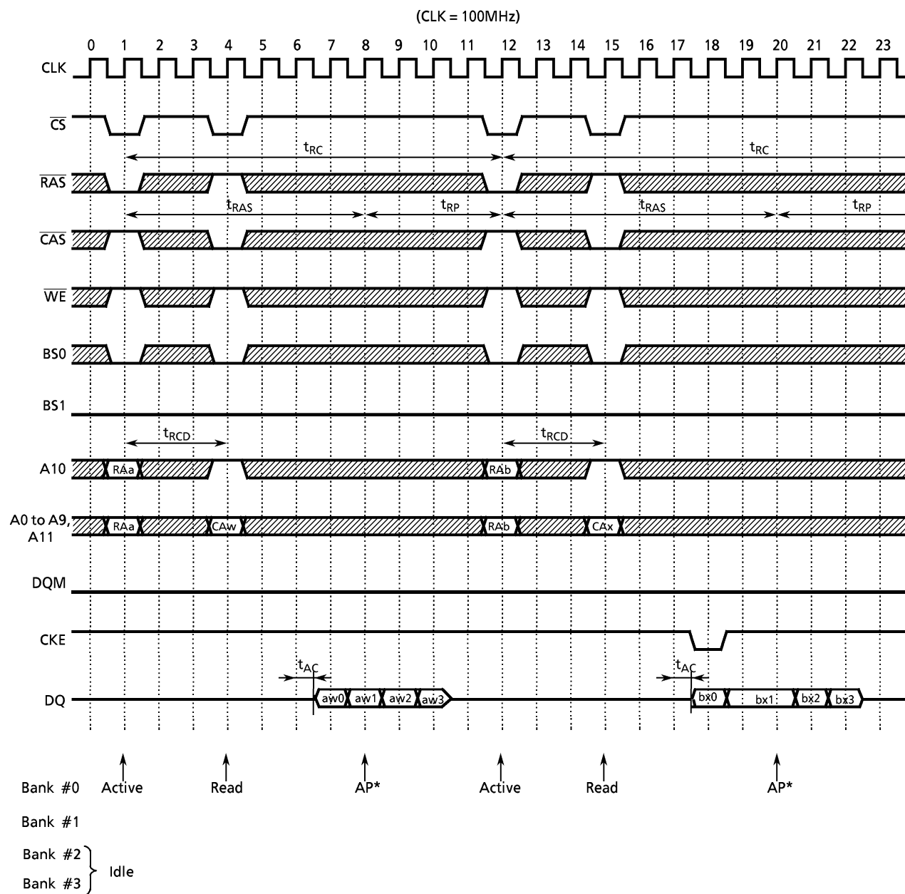
Figure 9. Auto Precharge Read (Burst Length=4, \overline{\text{CAS}} Latency=3)
