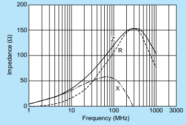
BLM31PG121SN1
