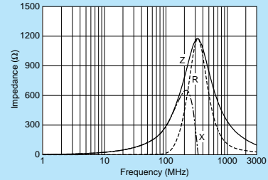
BLM18BB331SN1
