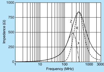
BLM18BB221SN1
