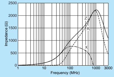
BLM03HD102SN1
