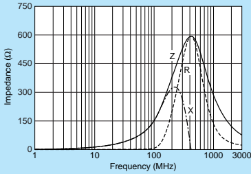
BLM18BB151SN1
