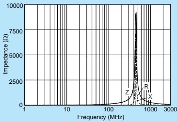
BLM18BA121SN1
