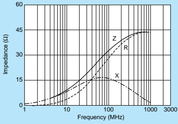
BLM31PG330SN1
