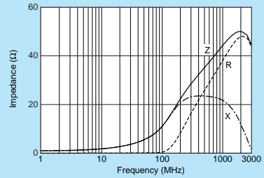
BLM18BB100SN1
