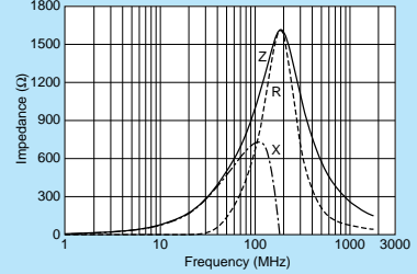
BLM21BD102SN1
