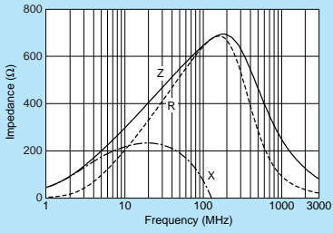
BLM18RK601SN1
