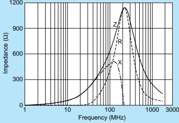
BLM21BD601SN1
