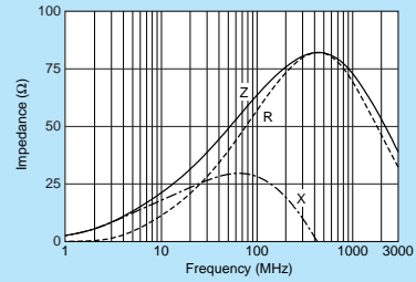
BLM18PG600SN1
