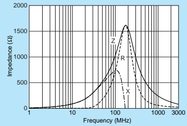
BLM18BD102SN1
