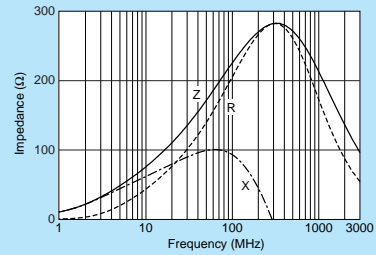
BLM18PG221SN1
