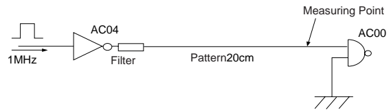
Measuring Circuits
