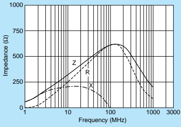
BLM21RK601SN1
