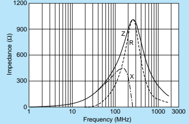
BLM21BD471SN1
