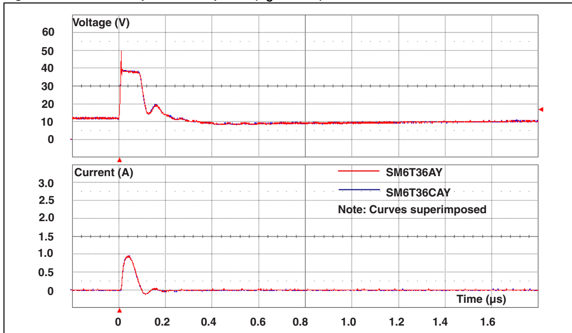
Figure 9. ISO 7637-2 pulse 3b response ( V_S = 100\text{ V} )
