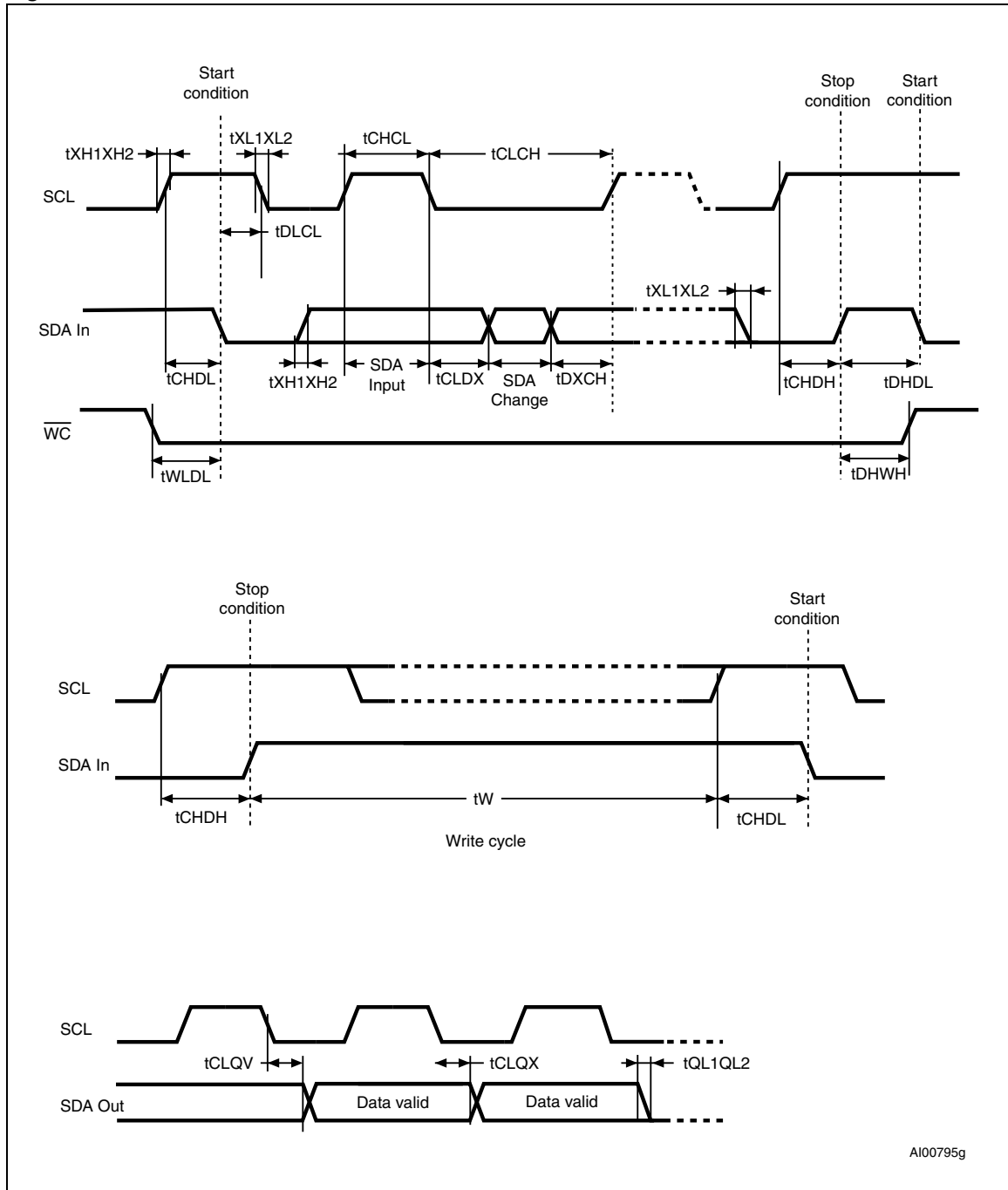
Figure 13. AC waveforms
