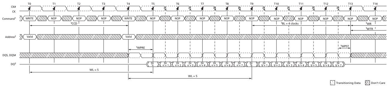
Figure 79: Consecutive WRITE (BL8) to WRITE (BL8)
