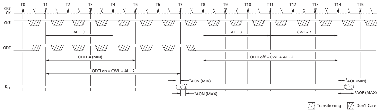
Figure 108: Synchronous ODT
