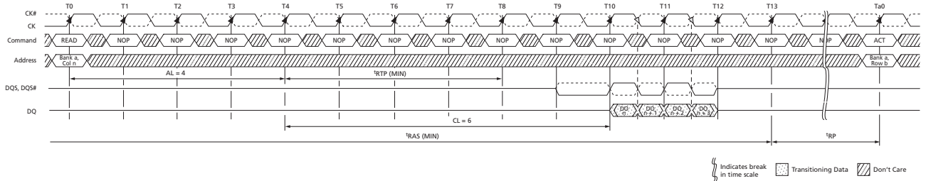
Figure 70: READ with Auto Precharge (AL = 4, CL = 6)
