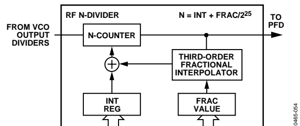
Figure 54. RF Fractional-N Divider
