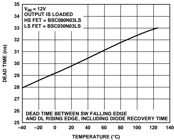
Figure 11. Dead Time vs. Temperature
