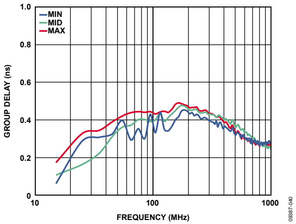
Figure 43. Group Delay vs. Frequency at Max, Mid, and Min Gain Outputs
