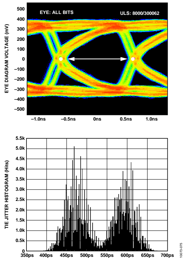
Figure 71. Data Eye for LVDS Outputs in ANSI-644 Mode with Trace Lengths Less than 24 Inches on Standard FR-4 Material, External 100 Ω Far-End Termination Only
