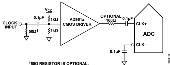
150 \Omega RESISTOR IS OPTIONAL. Figure 66. Single-Ended 1.8 V CMOS Input Clock (Up to 200 MHz)
