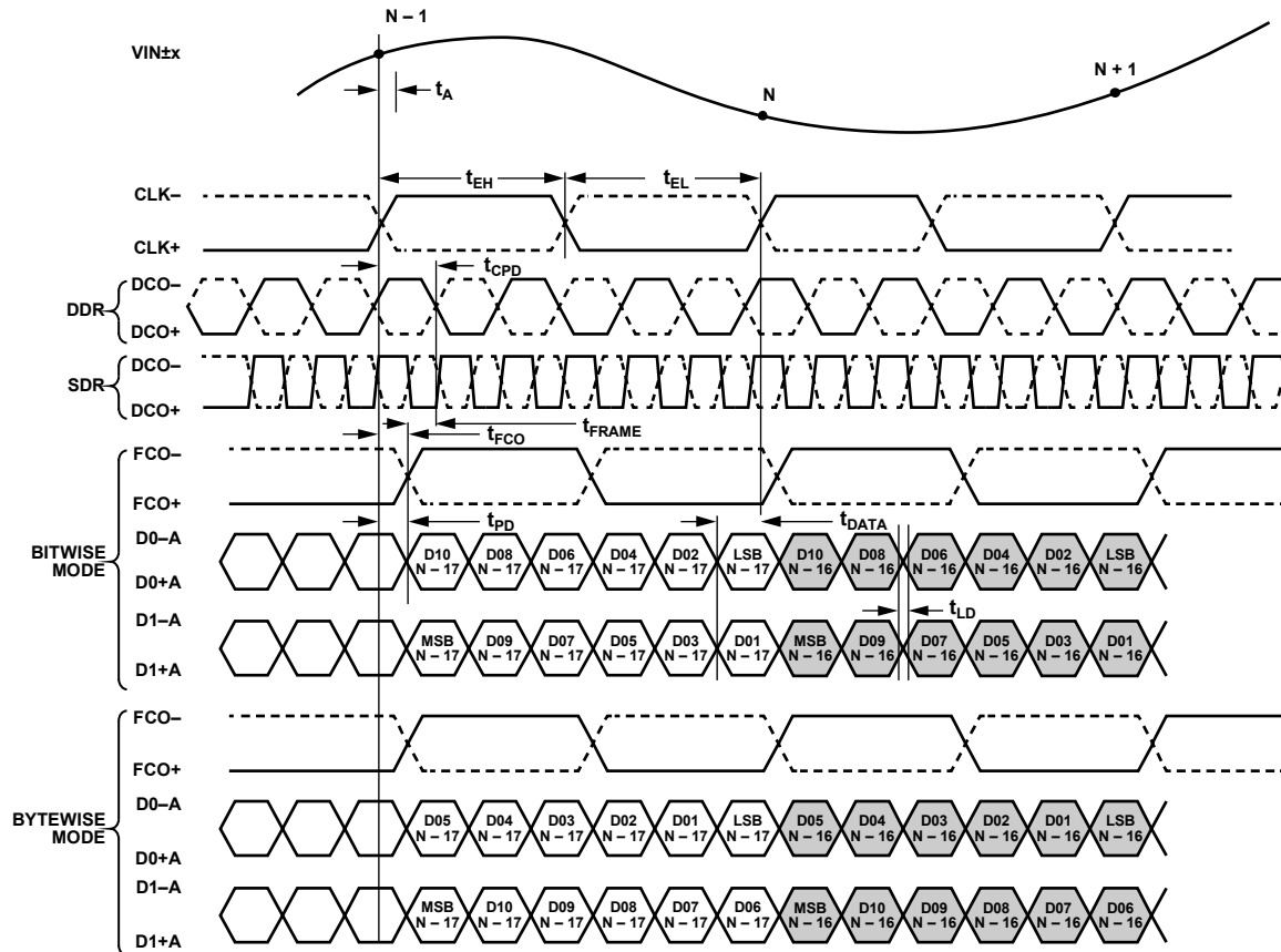
Figure 2. 12-Bit DDR/SDR, Two-Lane, 1x Frame Mode (Default)
