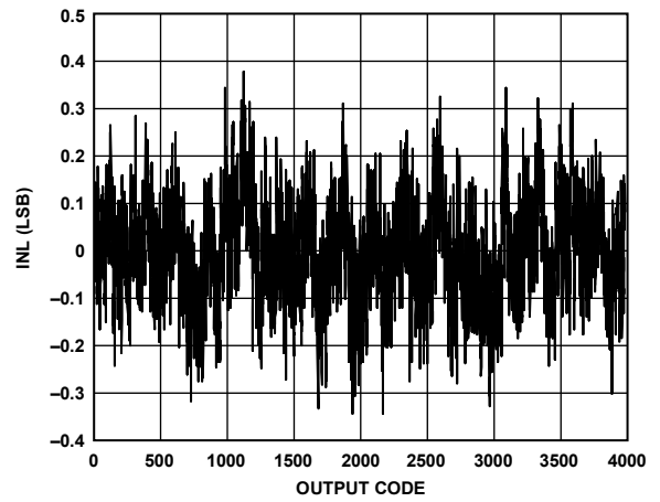
Figure 40. INL, f_{IN} = 9.7 MHz, f_{SAMPLE} = 125 MSPS
