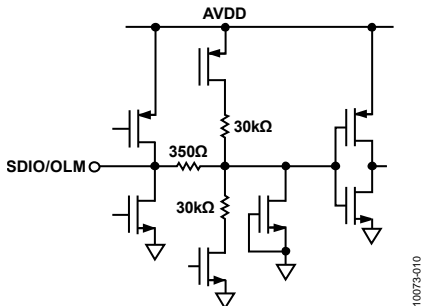
Figure 48. Equivalent SDIO/OLM Input Circuit
