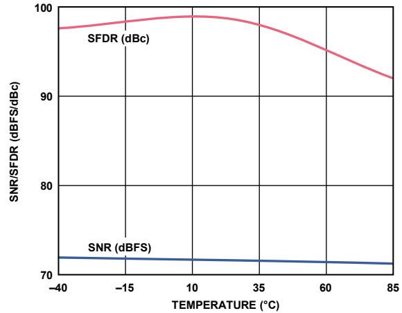
Figure 39. SNR/SFDR vs. Temperature, f_{IN} = 10.3 MHz, f_{SAMPLE} = 125 MSPS
