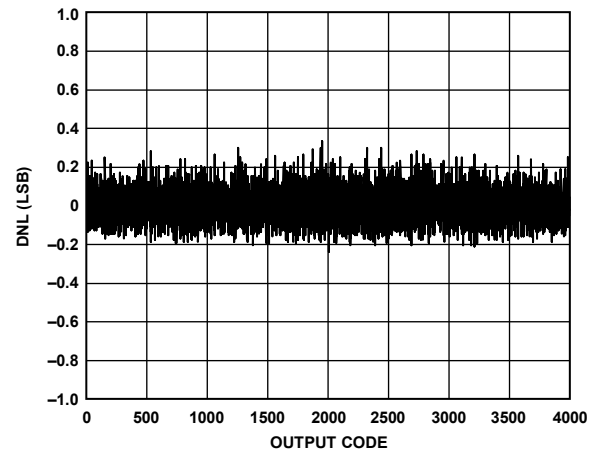
Figure 41. DNL, f_{IN} = 9.7 MHz, f_{SAMPLE} = 125 MSPS
