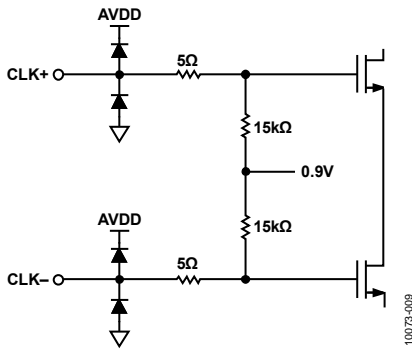
Figure 47. Equivalent Clock Input Circuit
