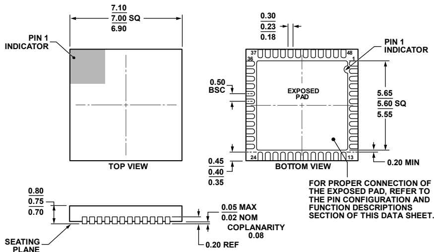
COMPLIANT TO JEDEC STANDARDS MO-220-WKKD. Figure 76. 48-Lead Lead Frame Chip Scale Package [LFCSP_WQ] 7 mm × 7 mm Body, Very Very Thin Quad (CP-48-13) Dimensions shown in millimeters
