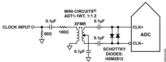
Figure 58. Transformer-Coupled Differential Clock
