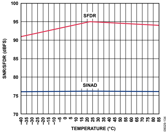
Figure 34. SINAD/SFDR vs. Temperature, f_{IN} = 97.3 MHz, 2.5 V p-p FS, AD9467-200
