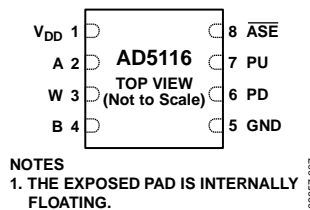
Figure 7. Pin Configuration
