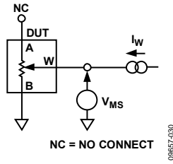
Figure 32. Resistor Position Nonlinearity Error (Rheostat Operation: R-INL, R-DNL)
