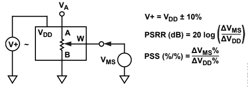
Figure 35. Power Supply Sensitivity (PSS, PSRR)
