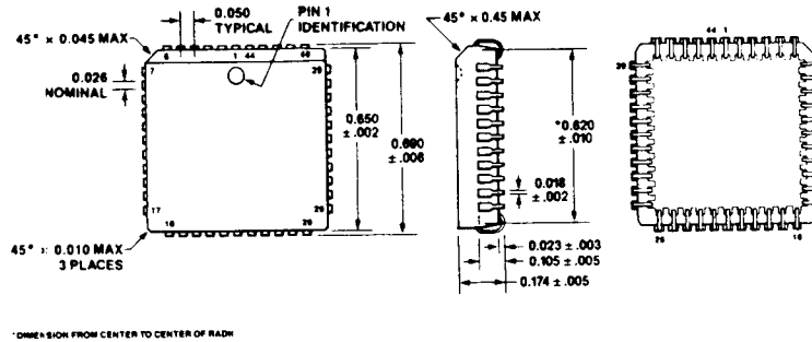
Bottom View
