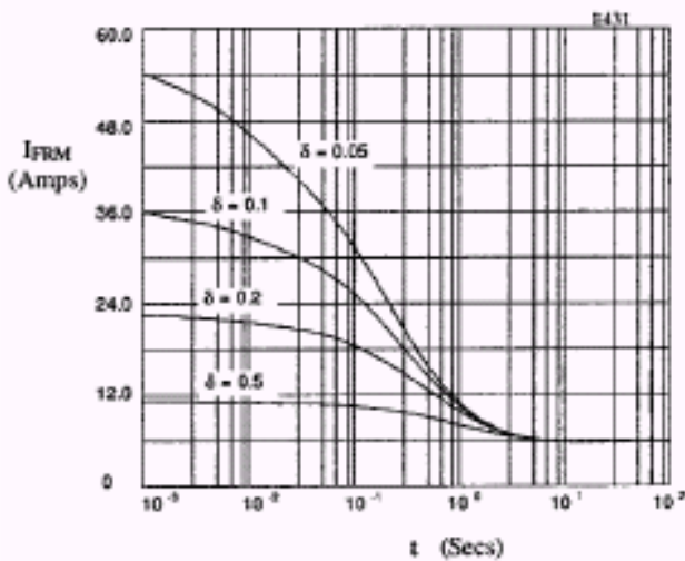
Fig 7. Typical repetitive forward current as a function of pulse width at 55°C; R_{\theta JL} = 20 °C/W; V_{RWM} during 1 - \delta .
