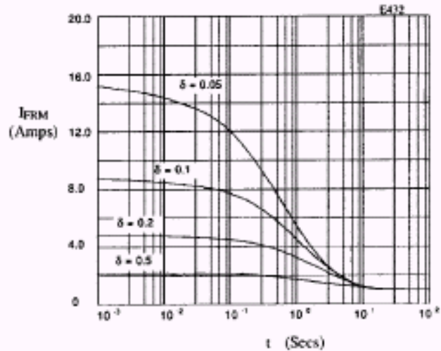
Fig 8. Typical repetitive forward current as a function of pulse width at 100°C; R_{\theta JL} = 80 °C/W; V_{RWM} during 1 - \delta .
