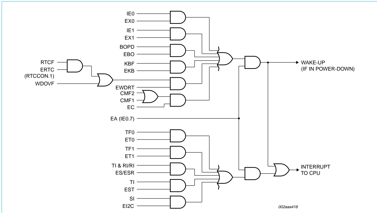
Fig 6. Interrupt sources, interrupt enables, and power-down wake-up sources.
