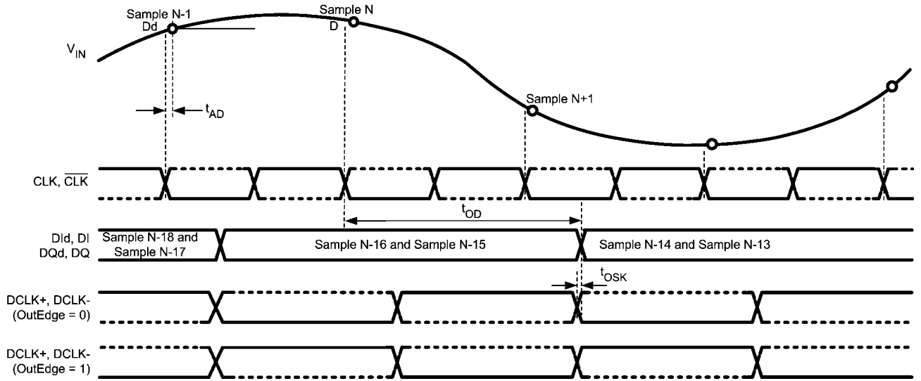
FIGURE 3. ADC08D500 Timing — SDR Clocking
