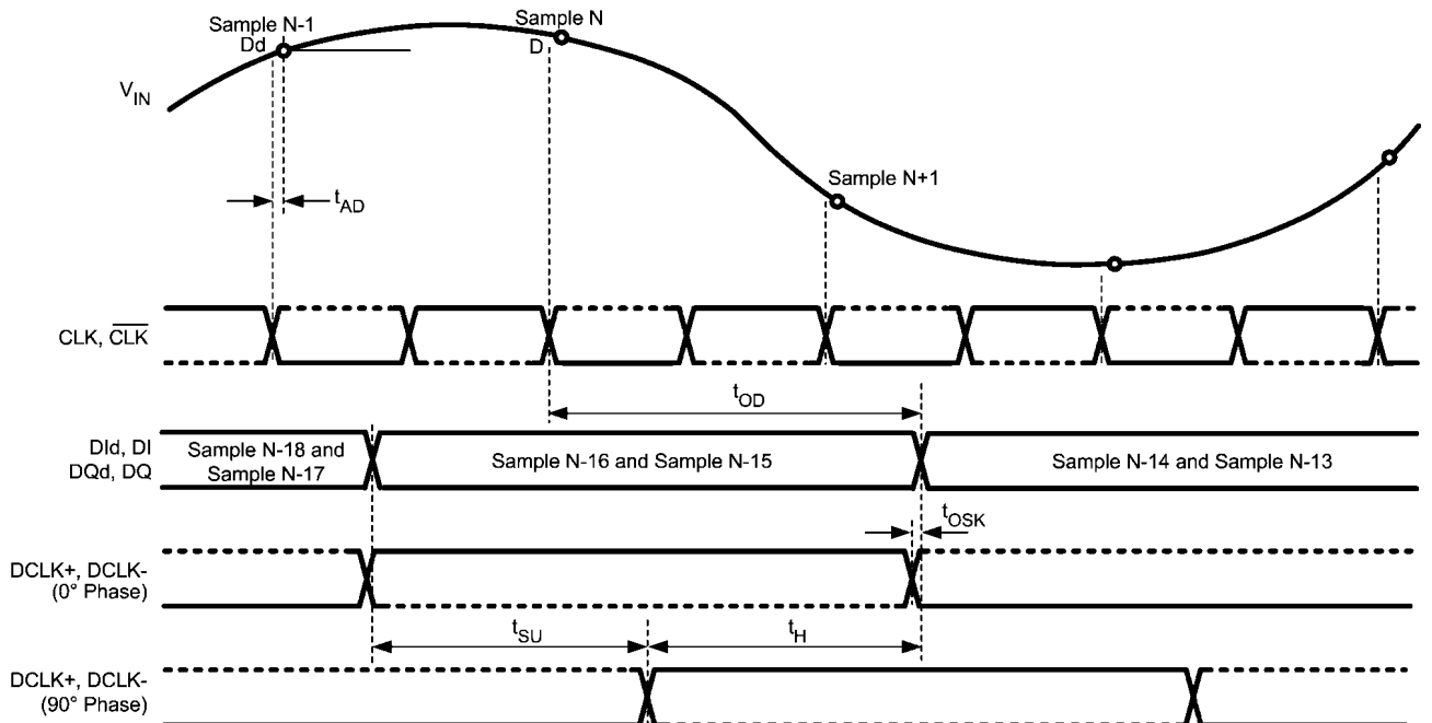
FIGURE 4. ADC08D500 Timing — DDR Clocking
