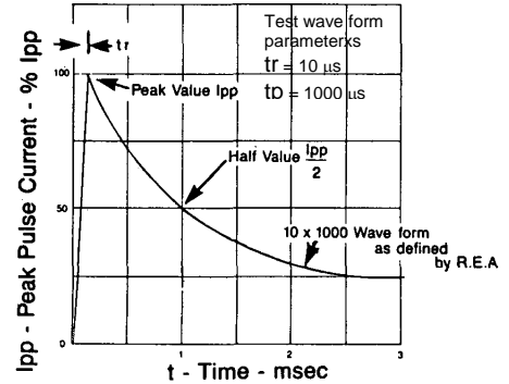
FIGURE 2 PULSE WAVEFORM
