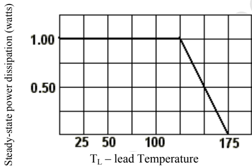
FIG. 3 Steady-state power derating curve
