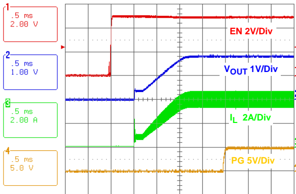
FIGURE 25. SOFT-START AT FULL LOAD
