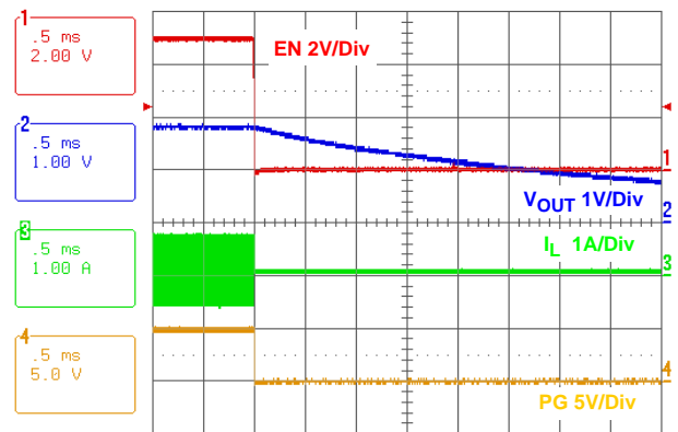
FIGURE 26. SOFT-DISCHARGE SHUTDOWN
