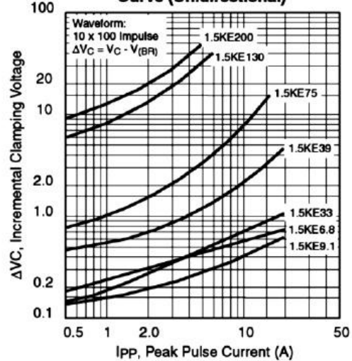
Fig. 8 – Incremental Clamping Voltage Curve (Unidirectional)
