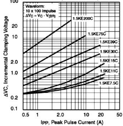
Fig. 10 – Incremental Clamping Voltage Curve (Bidirectional)
