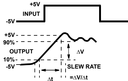
FIGURE 2. SLEW RATE
