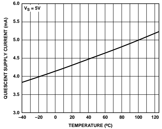
Figure 39. Supply Current per Amplifier vs. Temperature
