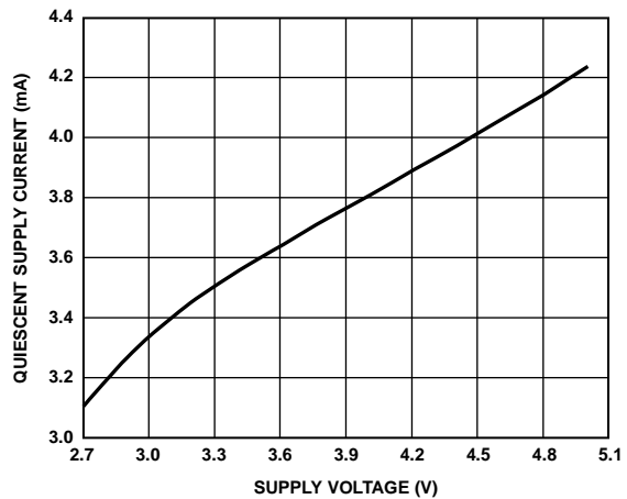
Figure 40. Supply Current per Amplifier vs. Supply Voltage
