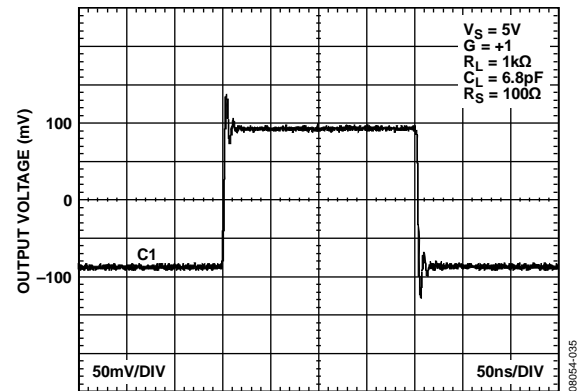
Figure 48. 200 mV Step Response, C_L = 50 \text{ pF}
