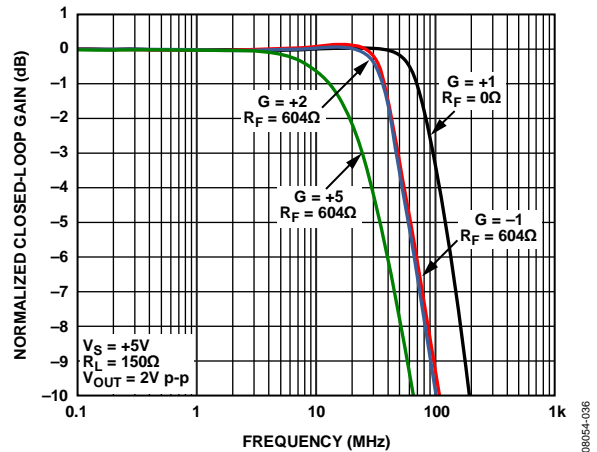
Figure 13. Large Signal Frequency Response vs. Gain, V_S = 5V
