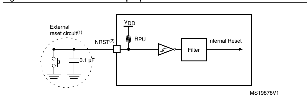
Figure 19. Recommended NRST pin protection
