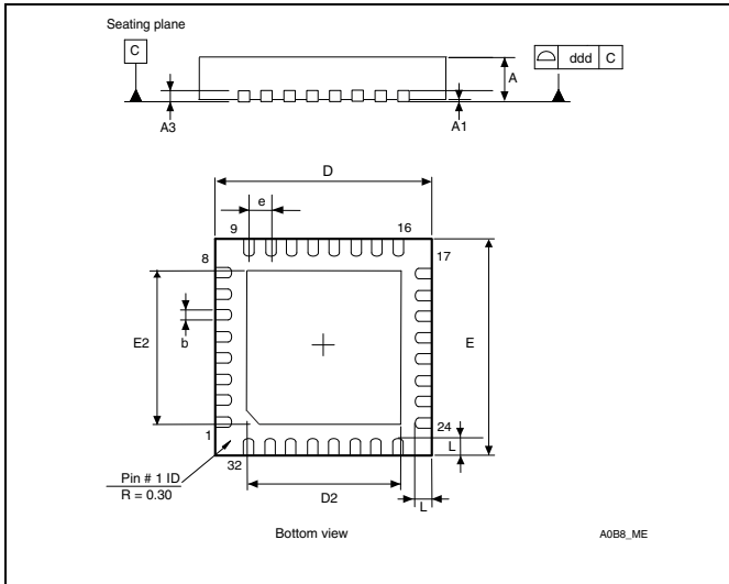
Figure 30. UFQFPN32 - 32-lead ultra thin fine pitch quad flat no-lead package outline (5 x 5) (1)(2)(3)
