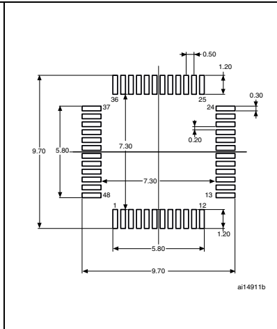
Figure 29. Recommended footprint (1)(2)
