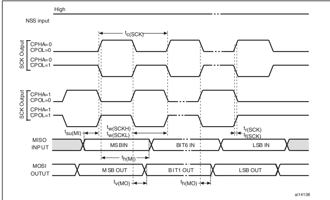
Figure 23. SPI timing diagram - master mode (1)
