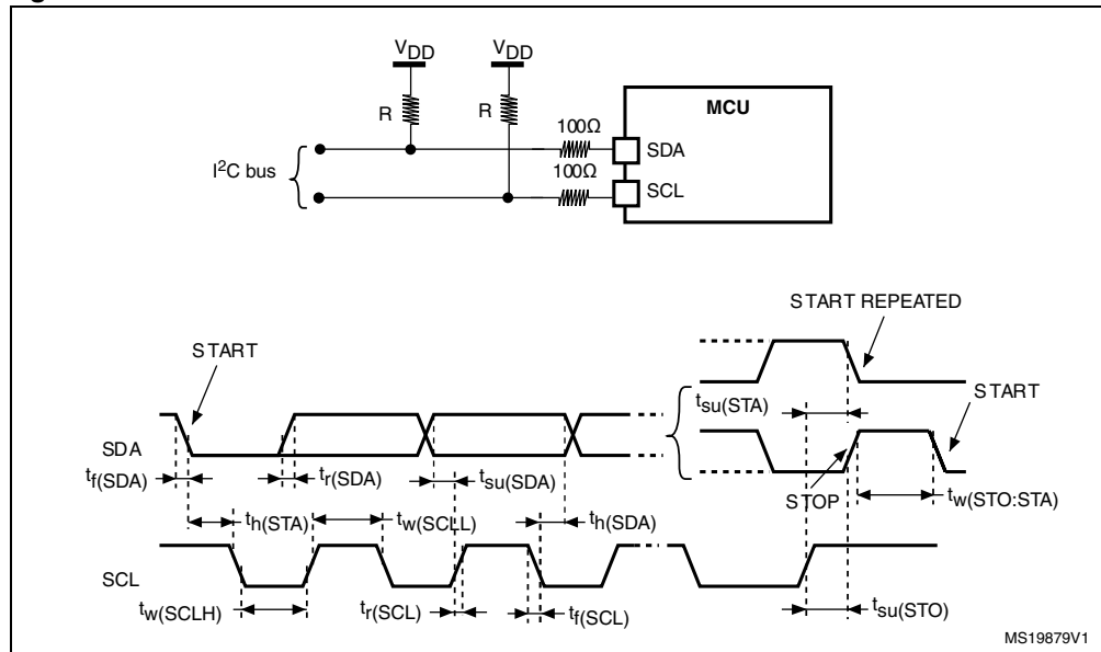
Figure 20. I2C bus AC waveforms and measurement circuit
