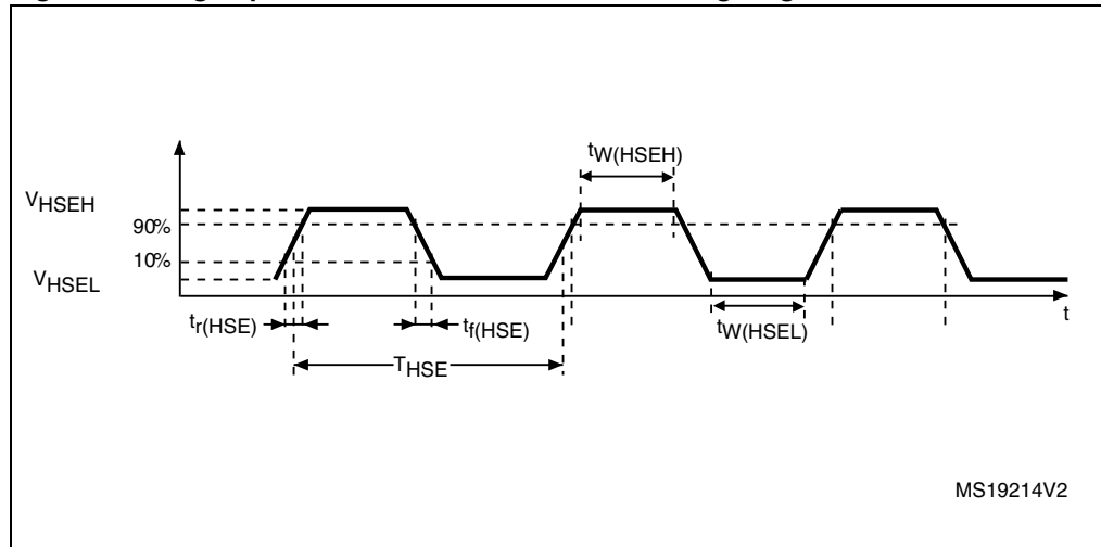
Figure 10. High-speed external clock source AC timing diagram
