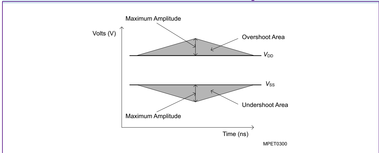
FIGURE 4 AC Overshoot / Undershoot Diagram for Address and Control Pins
