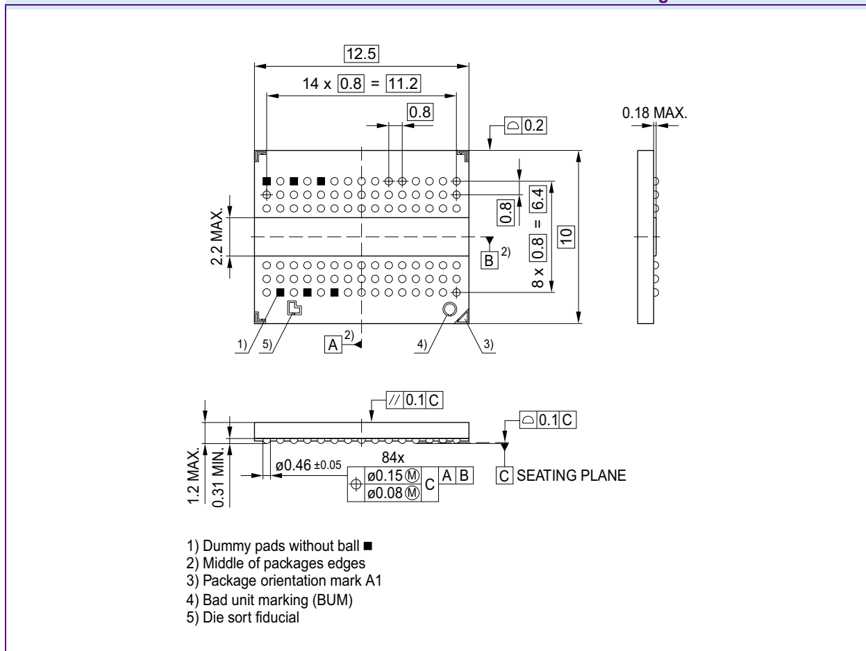
FIGURE 9 Package Outline PG-TFBGA-84
