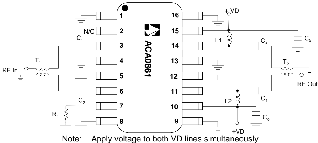
Figure 1. Test Circuit
